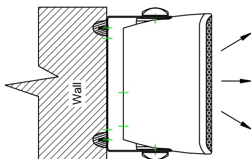
Wall fastening of the loudspeaker
