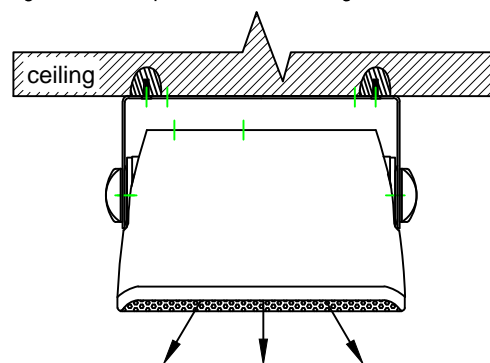
Fastening of the loudspeaker on the ceiling
